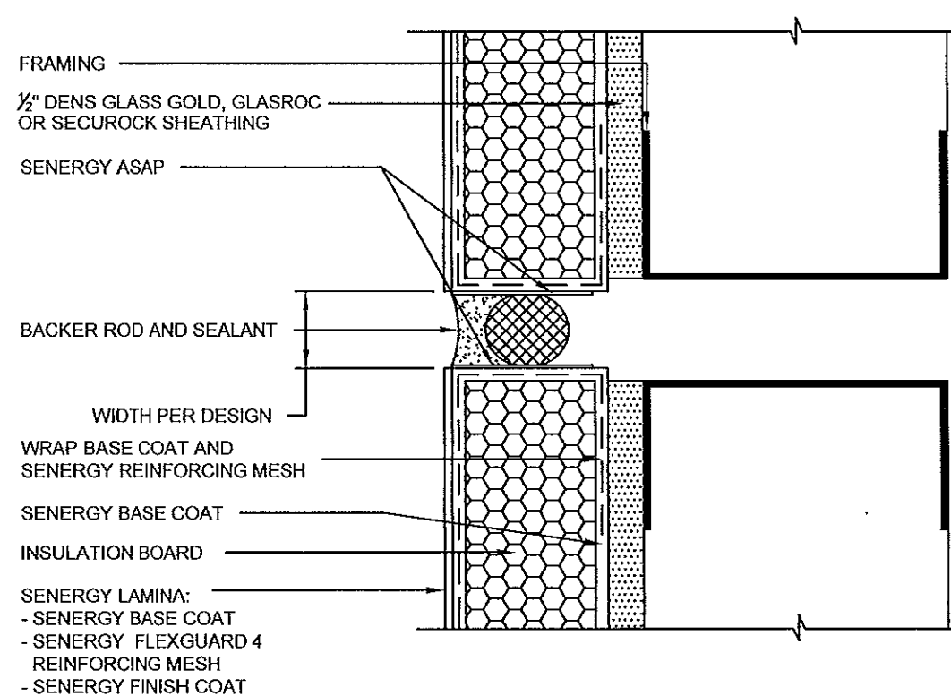
EXPANSION JOINT DETAIL
