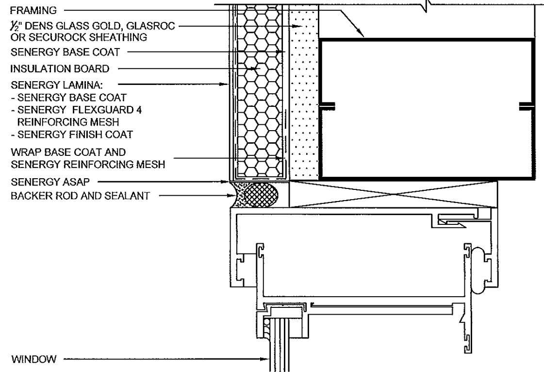
WINDOW JAMB DETAIL (FLUSH)
